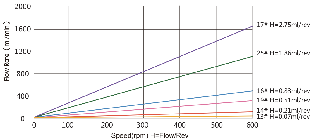
KZ15 Three-roller Pump-head
